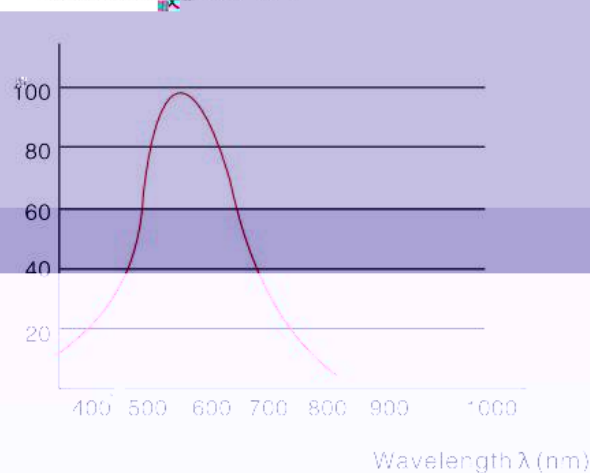
Spectrum Response Characteristic, 光谱响应特性曲线
